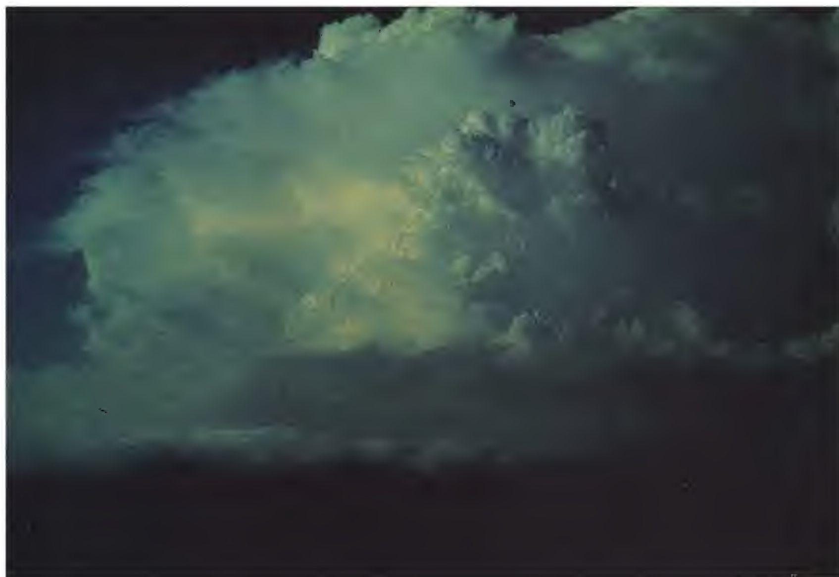
Figure 15. The glaciated anvil and the “soft” updraft tower (behind the towering cumulus in the foreground) suggest a lack of severity. Photo - National Severe Storms laboratory (NSSL).
